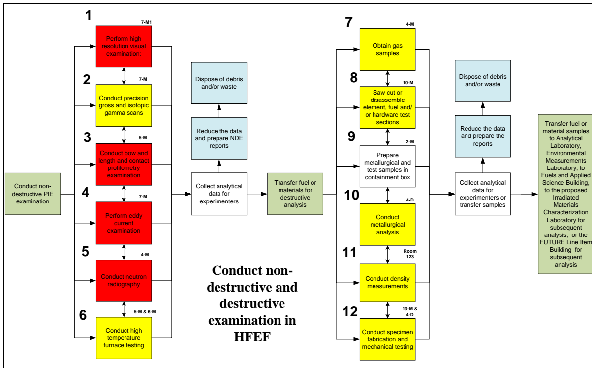
Figure 2. Hot Fuel Examination Facility PIE Processes
